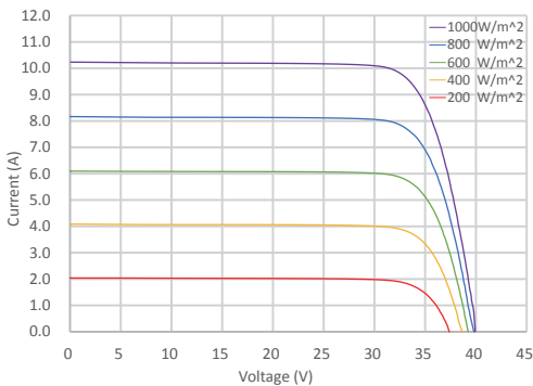
I-V Curves under Different Irradiance Levels
